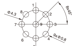
9Pins Female
