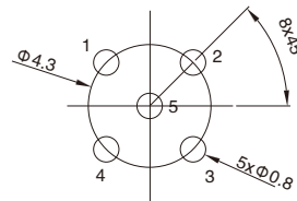
5Pins Female
